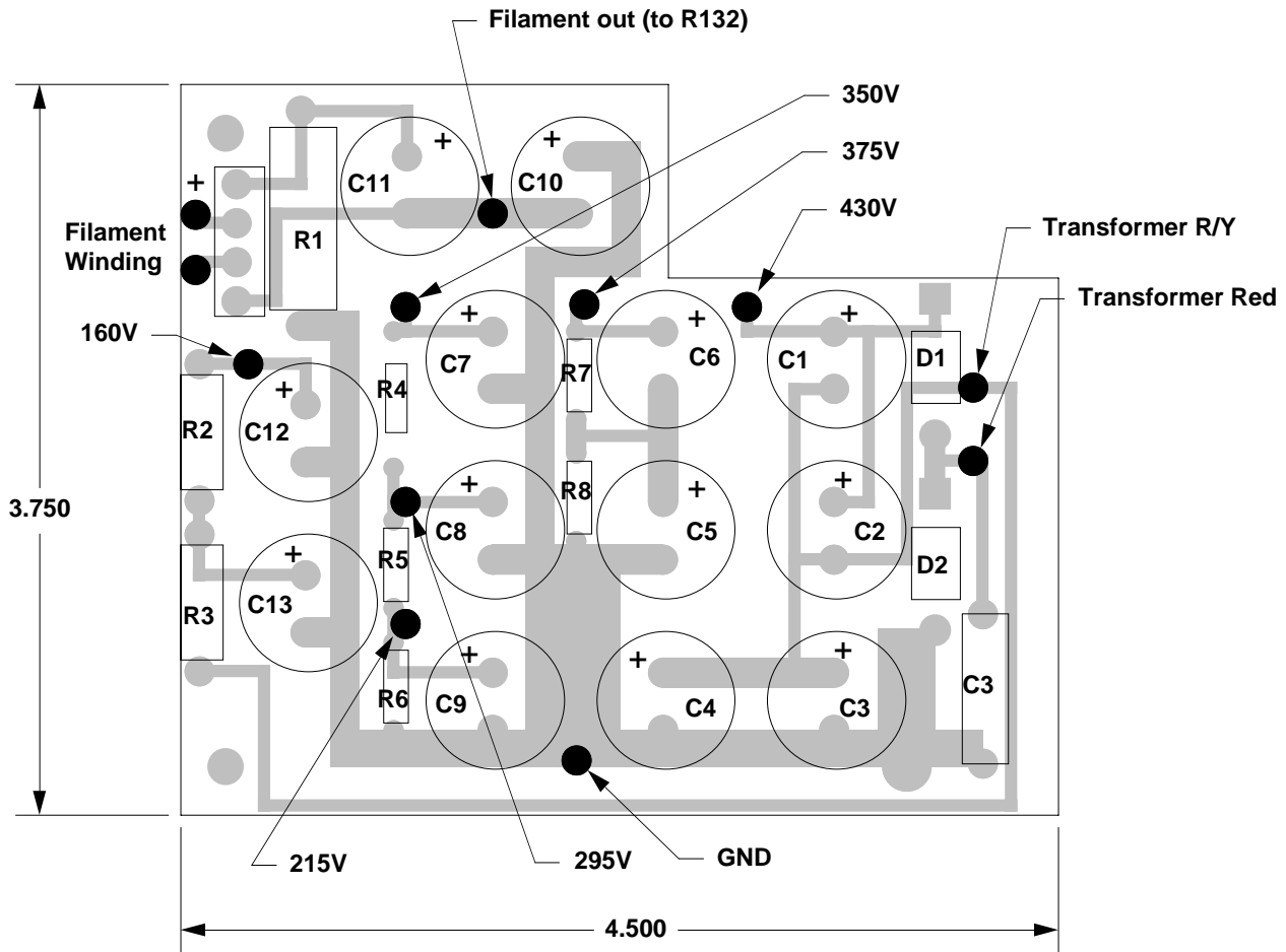
Capacitor Board Parts Placement and Wiring Guide
