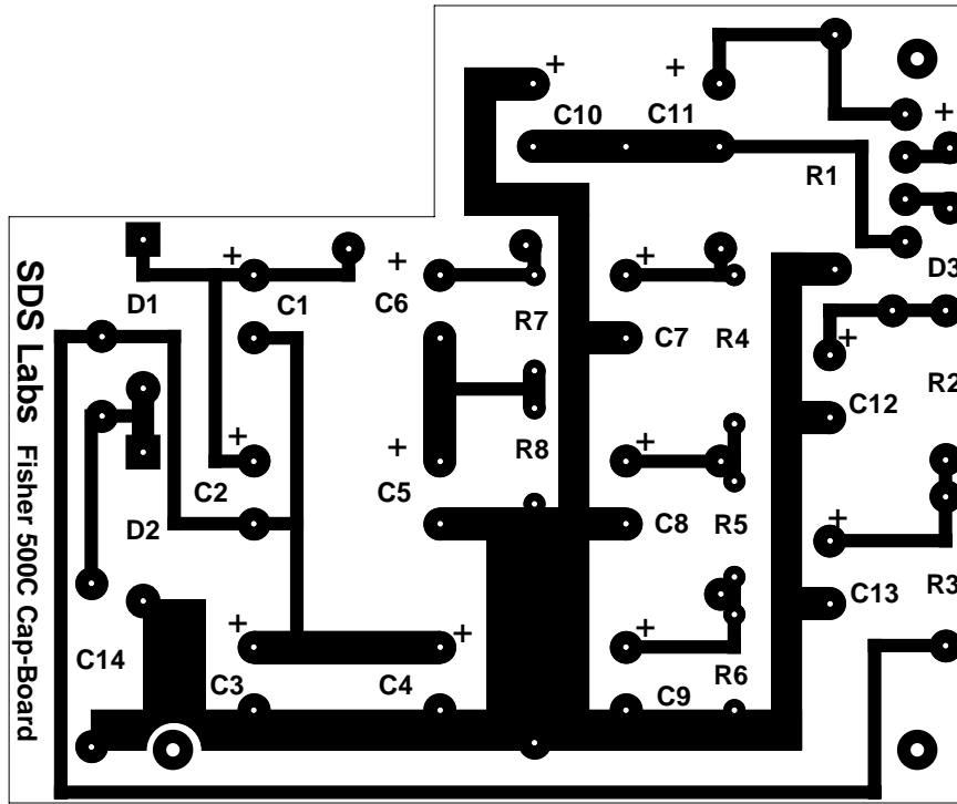
Capacitor Board Layout
