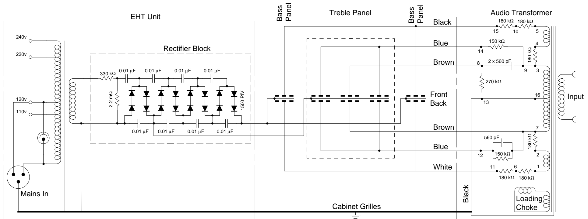
Quad ESL Schematic by SDS Labs June 26, 1997
